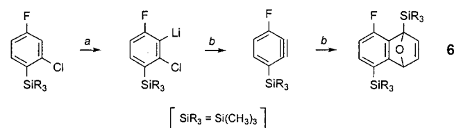
Scheme 4. Perfect regioselective cycloaddition between 3-fluoro-6-trimethylsilyl-1,2-didehydrobenzene and 2-(trimethylsilyl)furan. a : sec -Butyllithium in THF at -75^{\circ}\text{C} . b : Addition of 2 equiv. of 2-(trimethylsilyl)furan and rapid heating to +60^{\circ}\text{C} .
