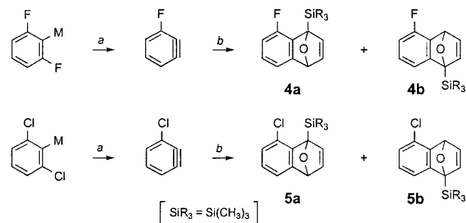
Scheme 3. Trapping of 3-fluoro- and 3-chloro-1,2-didehydrobenzene with 2-(trimethylsilyl)furan. a : M = H; sec -butyllithium in THF at -75^{\circ}\text{C} ( \Rightarrow M = Li). b : Transfer through Teflon tubing into a solution of 2-(trimethylsilyl)furan in THF.
