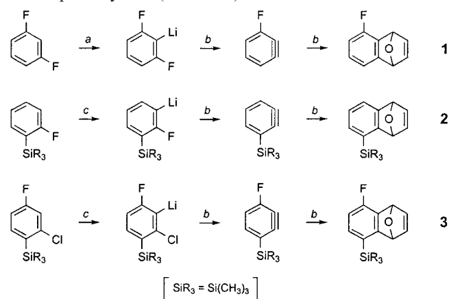
Scheme 2. Trapping of 3-fluoro-1,2-didehydrobenzene, 3-trimethylsilyl-1,2-didehydrobenzene, and 3-fluoro-6-trimethylsilyl-1,2-didehydrobenzene with furan. a : sec -Butyllithium in tetrahydrofuran (THF) at -75^{\circ}\text{C} . b : Transfer through Teflon tubing into furan kept at +25^{\circ}\text{C} . c : Butyllithium in THF at -75^{\circ}\text{C} .
